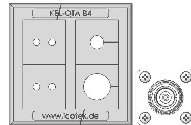
Cable Entry & Antenna Cable Connector
